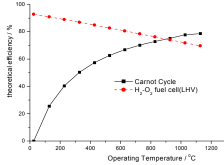
Figure 9. The theoretical efficiency of H_2-O_2 fuel cell and Carnot cycle versus temperature
