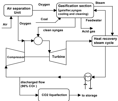
Figure 1. Flowchart of the semi-closed cycle IGCC system with CO 2 recovery
