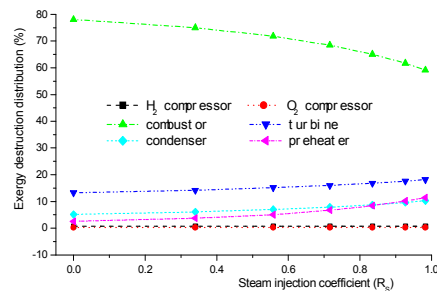
Figure 7. Effect of R_S on exergy destruction distributions in H_2/O_2 cycle.
