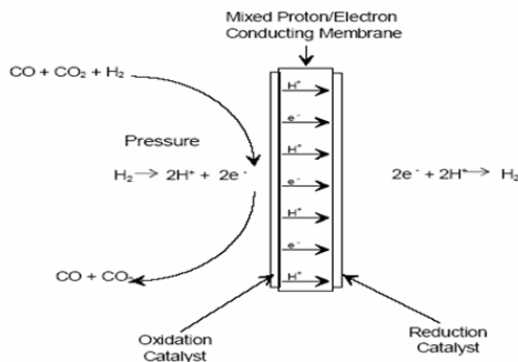
Figure 5. Schematic diagram of the ceramic proton membrane process for separating hydrogen from a mixture of gases
