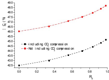
Figure 8. Variation of \eta_{ig} with R_s .
