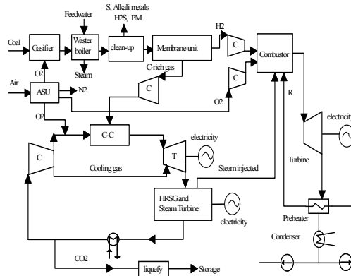
Figure 3. Flow diagram of IGCC system with steam-injected H 2 /O 2 cycle and CO 2 recovery
