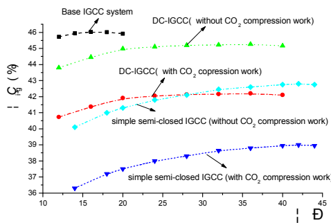
Figure 6. \eta_{ig} of different IGCC systems versus \pi
