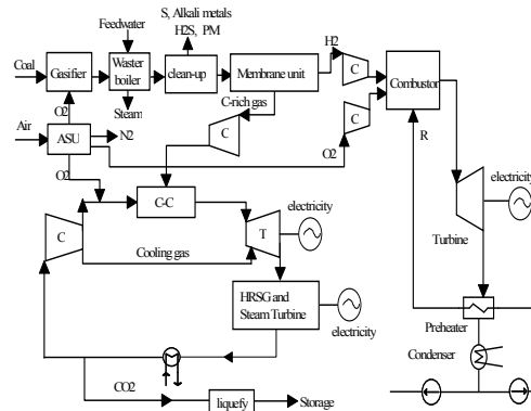
Figure 2. Flowchart of dual-cycle IGCC system with mixed H 2 /O 2 cycle and CO 2 recovery
