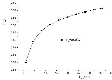
Figure 10. \eta_{fc} of H_2 - O_2 fuel cell versus P_{fc}
