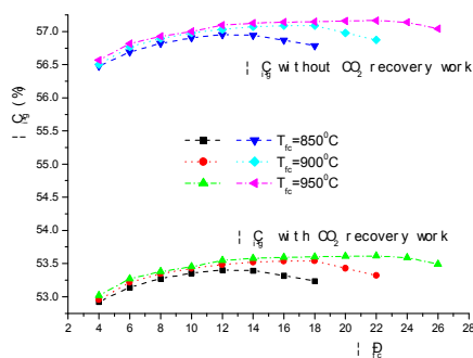
Figure 11. \eta_{ig} versus pressure ratio \pi_{gc}
