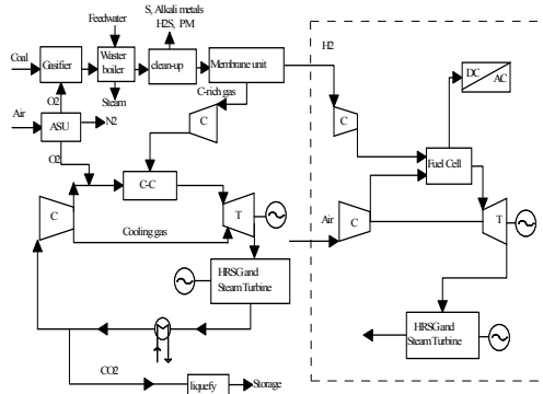
Figure 4. Flowchart of IGCC system with fuel cell combined cycle and CO 2 recovery
