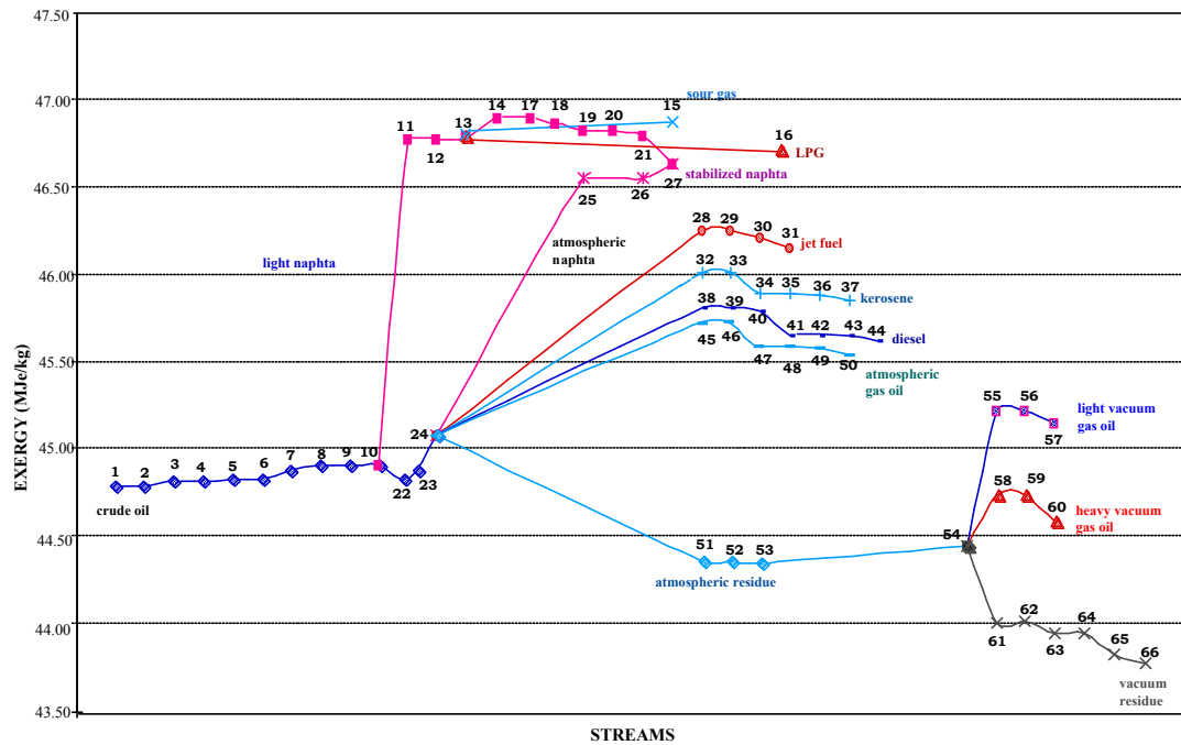
Figure 7. Specific exergy of process streams in a crude oil combined distillation unit.
