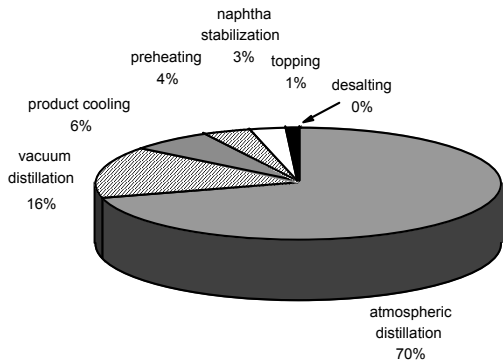
Figure 6. Distribution of improvement potentials.
