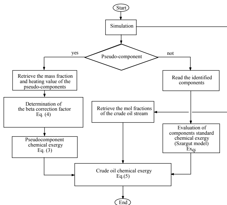
Figure 1. Calculation procedure of chemical exergy.
