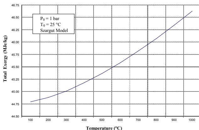
Figure 3. Total exergy of a mixture of Isthmus/Maya crude oils (48.5/51.5 wt%) at 1 bar.
