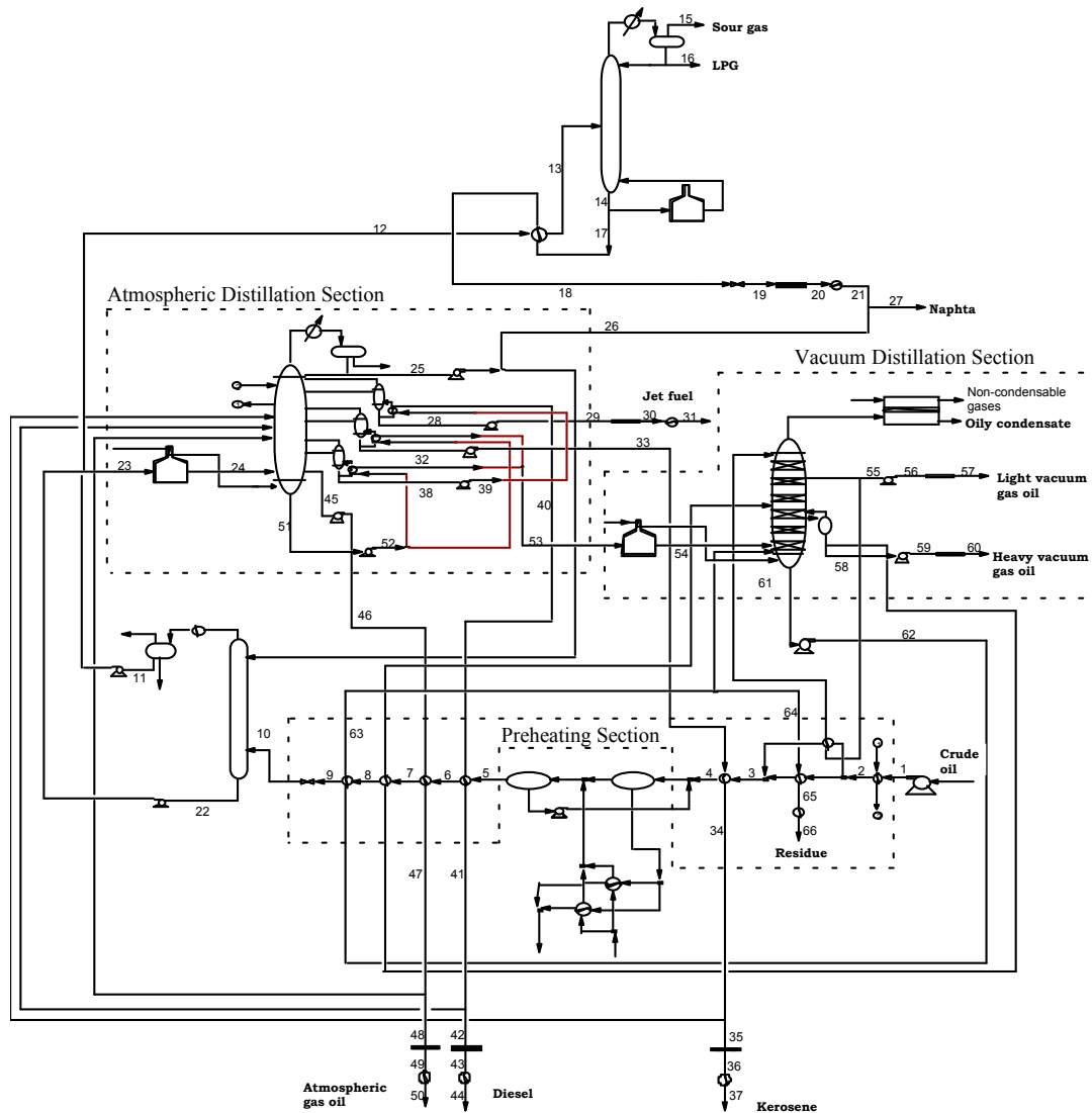
Figure 5. Crude oil combined distillation unit.
