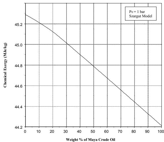
Figure 4. Chemical exergy of a mixture of Isthmus/Maya crude oils.
